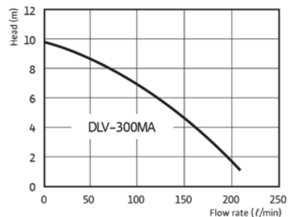
Performance Curve
